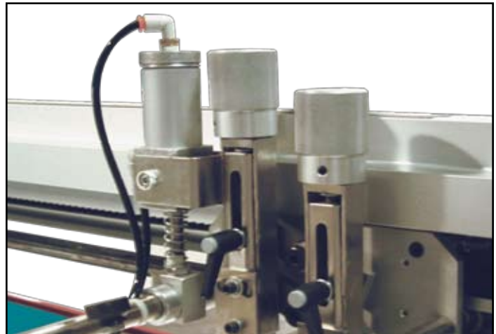
Pneumatic "Squeegeelizer" automatically adjusts for uniform squeegee pressure.
